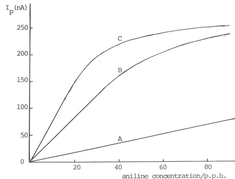
Figure 10. Calibration curves for aniline(after derivatization) using AdSV(DPP).Scan rate = 10 mV/s; t_{drop} = 1s ; E_{acc.} = -240 mV ; pH = 10; acc. time (min):A-0,B-1,C-2.
