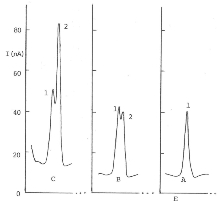
Figure 3. DPP determination of a mixture of D & C Red 6 (peak 1) and D & C Red 8 (peak 2). A - t_{step} = 5 s (scan rate = 2 mV/s); B - t_{step} = 1 s (scan rate = 10 mV/s); C - t_{step} = 0.2 s (scan rate = 50 mV/s). E_{set} = -350 mV; E_{end} = -900 mV.
